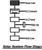
Solar System Flow Diagram
