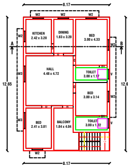
PROPOSED GROUND FLOOR PLAN
