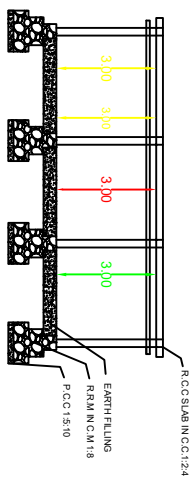
SECTION
