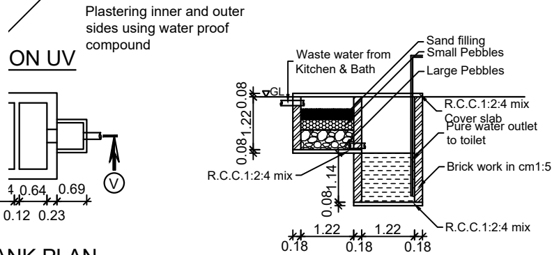
WASTE WATER RECYCLING SYSTEM
