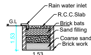
RAIN WATER HARVESTING PIT RW_H_CAPACITY_L=5000LTRS
