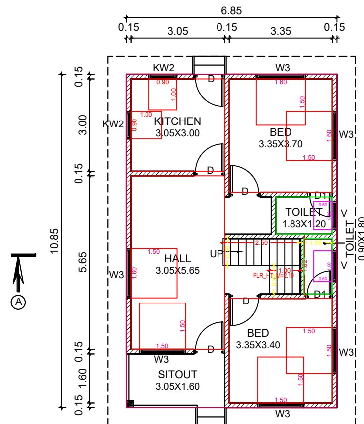
GROUND FLOOR PLAN TERRACE ROOF
