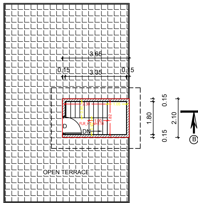
FIRST FLOOR PLAN SHEET ROOF
