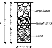
SECTION OF RAIN WATER COLLECTION PITS (NTS)
