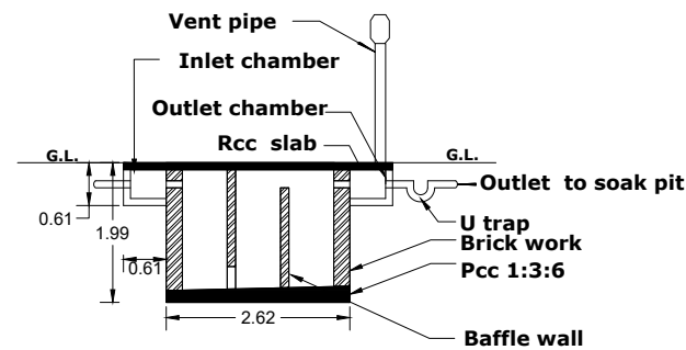
SECTION ON SR
