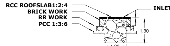
RAIN WATER HARVEST TRENCH
