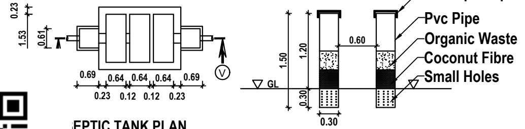
PIPE COMPOST PIT
