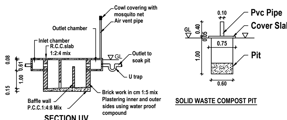
SECTION UV
