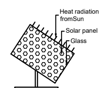
SOLAR SYSTEM
