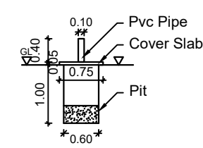
SOLID WASTE COMPOST PIT
