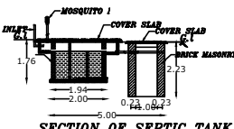
SECTION OF SEPTIC TANK
