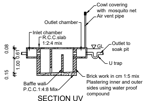
SECTION UV
