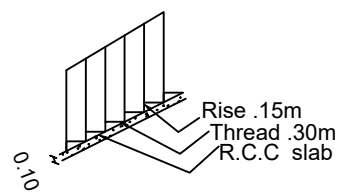
STAIRCASE DETAILS
