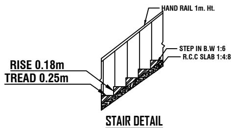
STAIR DETAIL
