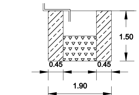
RAINWATER HARVESTING
