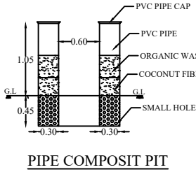
PIPE COMPOSITE PIT
