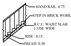
STAIR CASE SECTION
