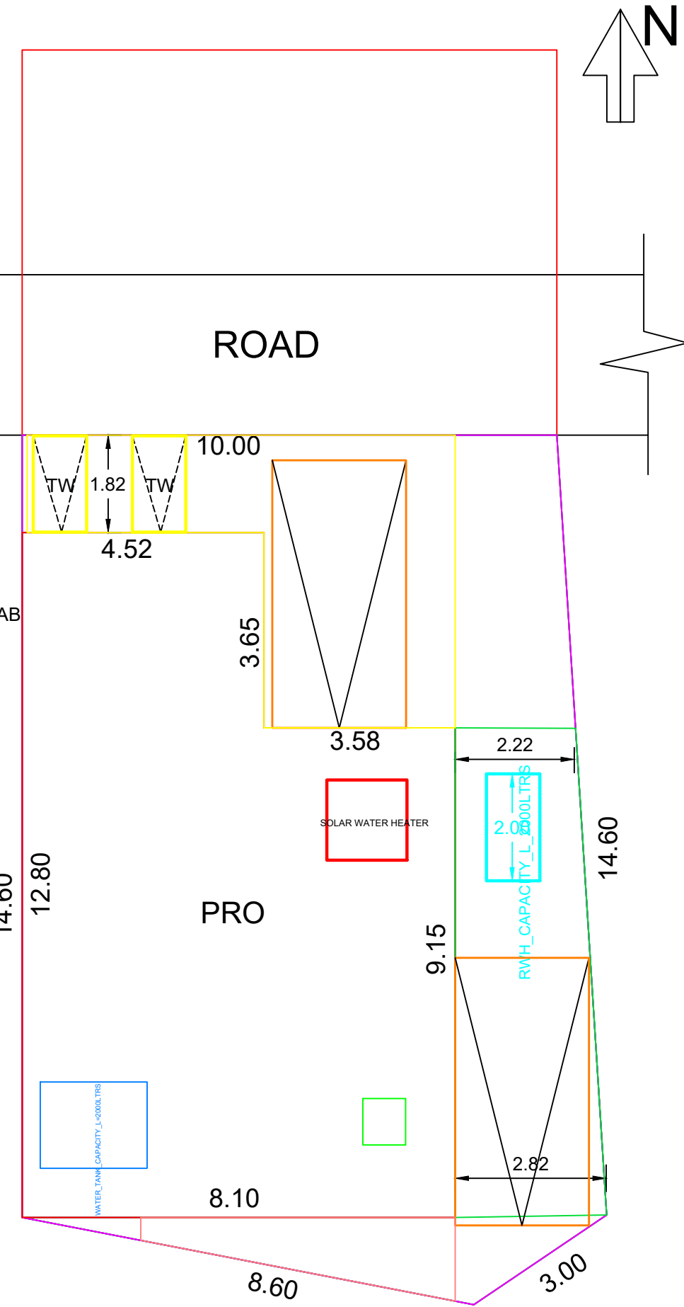
SITE PLAN
