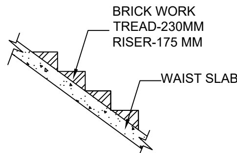
STAIRCASE DETAILS
