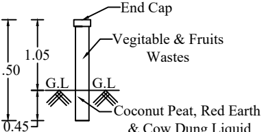
PIPE COMPOSTER
