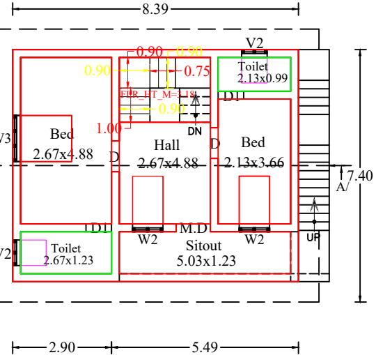
EXTENSION FIRST FLOOR PLAN
