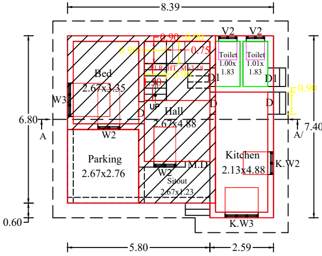
EXG. GROUND FLOOR PLAN
