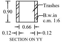
SECTION ON YY
