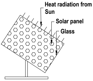
SOLAR SYSTEM
