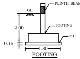
FOOTING
