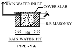
TYPE - 1 A
