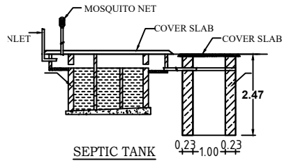
SEPTIC TANK
