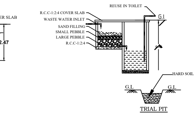
RECYCLING OF WASTE WATER KITCHEN & BATH ROOM
