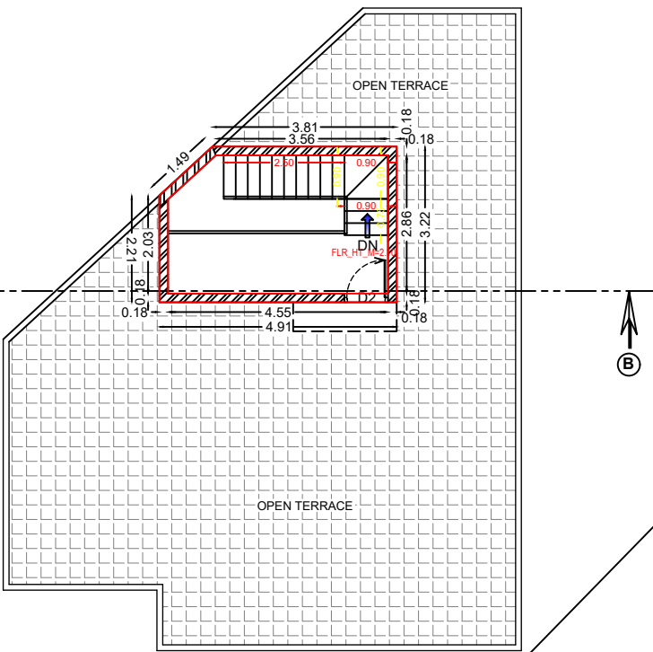
TOWER PLAN BUILTUP AREA =15.2 m 2 (163.55 sq.ft)
