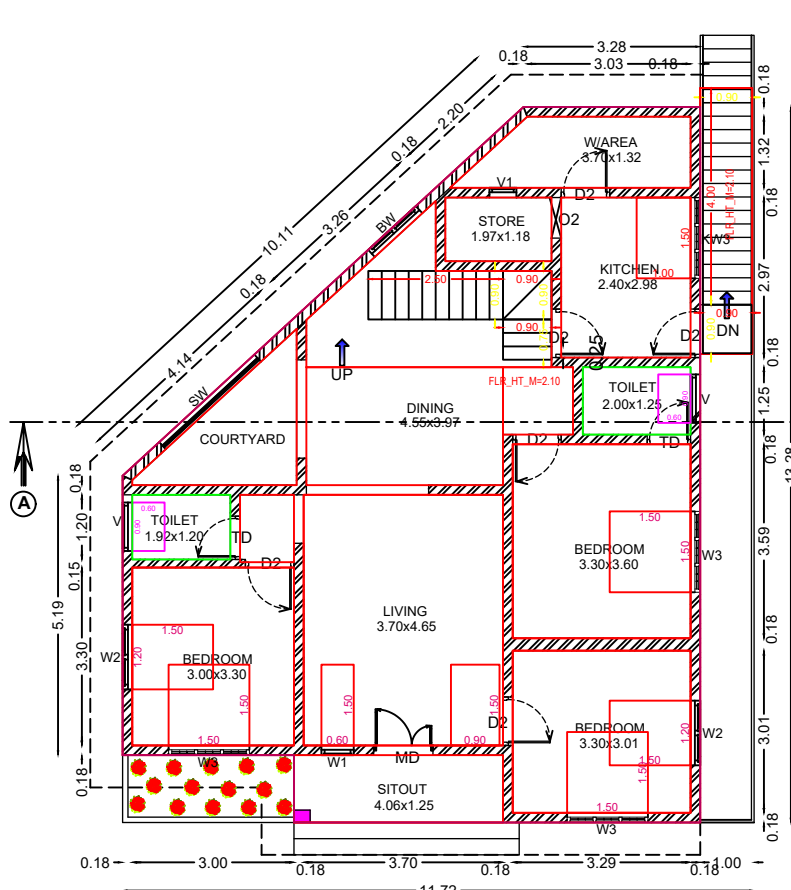
FIRST FLOOR PLAN BUILTUP AREA =112.9 m 2 (1214.80 sq.ft)
