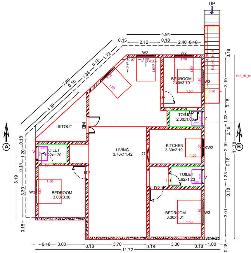
GROUND FLOOR PLAN BUILTUP AREA =106.8 m 2 (1149.17 sq.ft)
