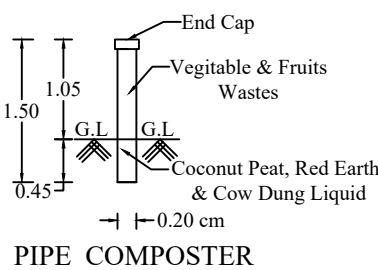
PIPE COMPOSTER
