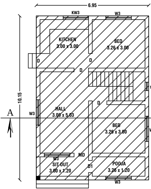
EX.GROUND FLOOR PLAN
