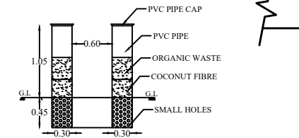
PIPE COMPOSITE PIT
