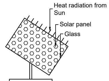
SOLAR SYSTEM
