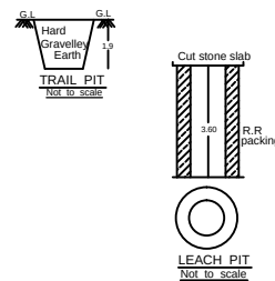
RAIN WATER HARVESTING ARRANGEMENT DRAWING TYPE - 1A
