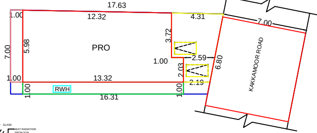
SITE PLAN
