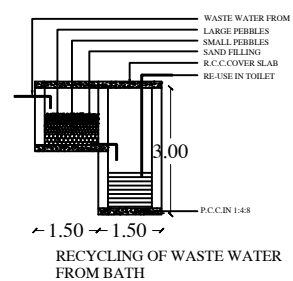
RECYCLING OF WASTE WATER FROM BATH
