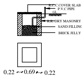
RAIN WATER HARVEST ARRANGEMENTS
