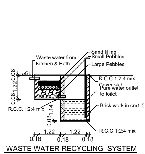
WASTE WATER RECYCLING SYSTEM
