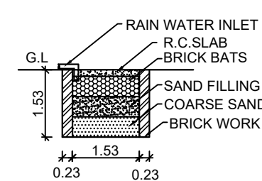
RAIN WATER HARVESTING TANK
