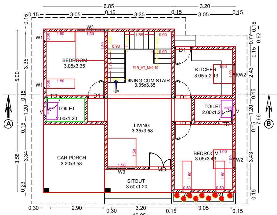
GROUND FLOOR PLAN BUILTUP AREA = 83.3 m 2 (896.31 sq.ft)
