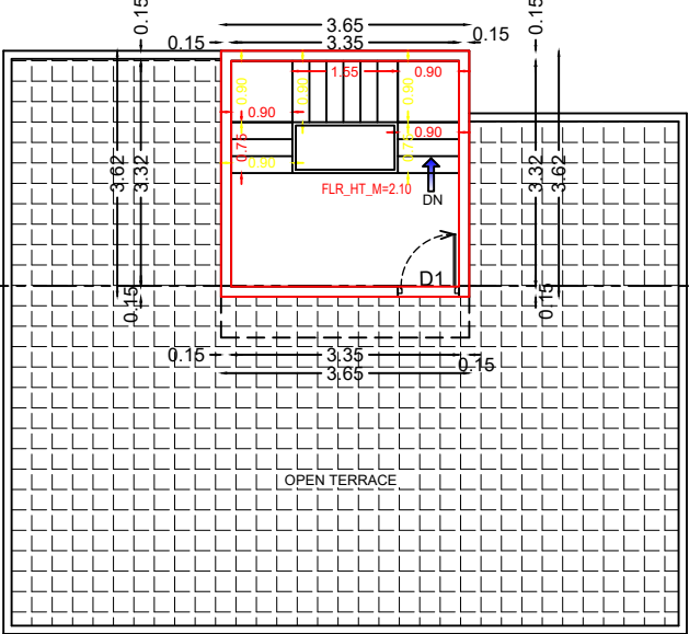
TOWER PLAN BUILTUP AREA = 13.2 m 2 (142.03 sq.ft)
