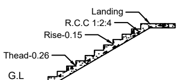
STAIR CASE DETAILS
