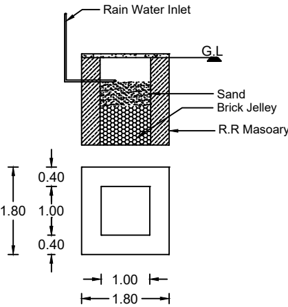
RAIN WATER HARVESTING DETAILS
