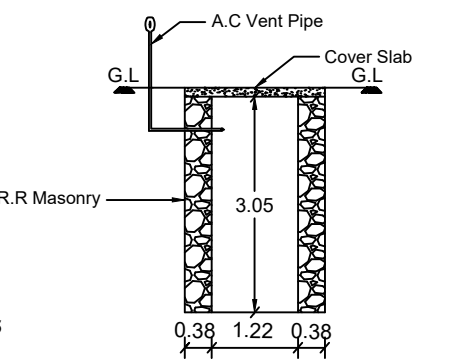
SOAKPIT SECTION
