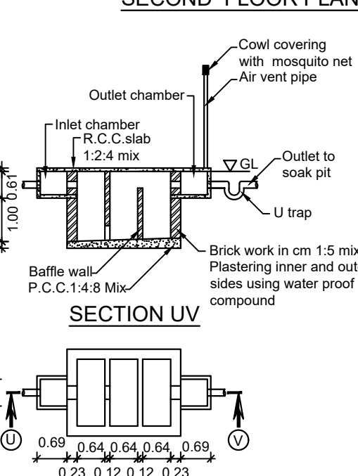
SEPTIC TANK PLAN
