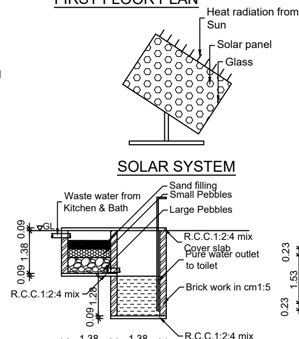
WASTE WATER RECYCLING SYSTEM
