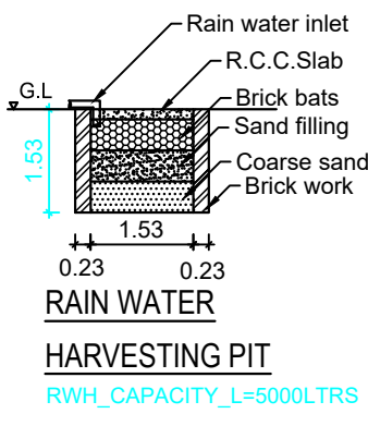
RAIN WATER HARVESTING PIT
