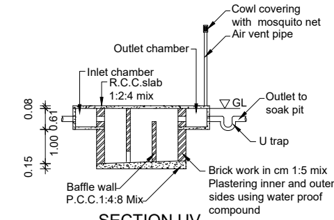
SECTION UV
