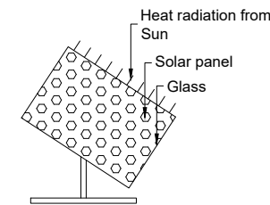
SOLAR SYSTEM
