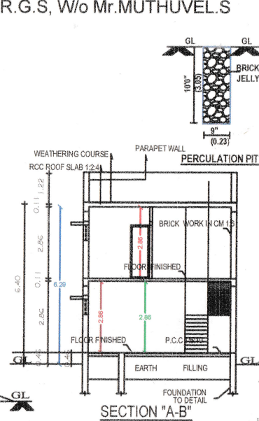
SECTION "A-B"
