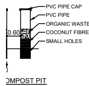
COMPOST PIT
