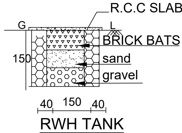
RWH TANK
