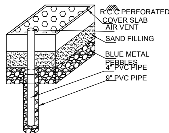
PERCOLATION BORE PIT
