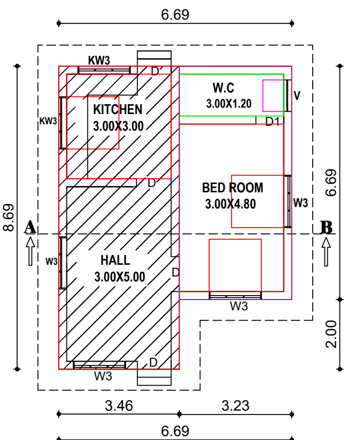
EXISTING & PROPOSED GROUND FLOOR- PLAN
