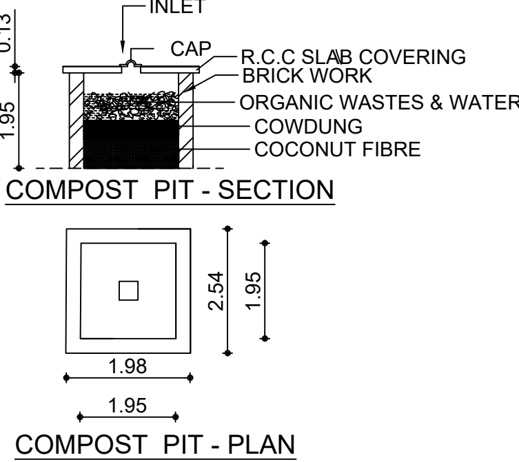
COMPOST PIT - PLAN
