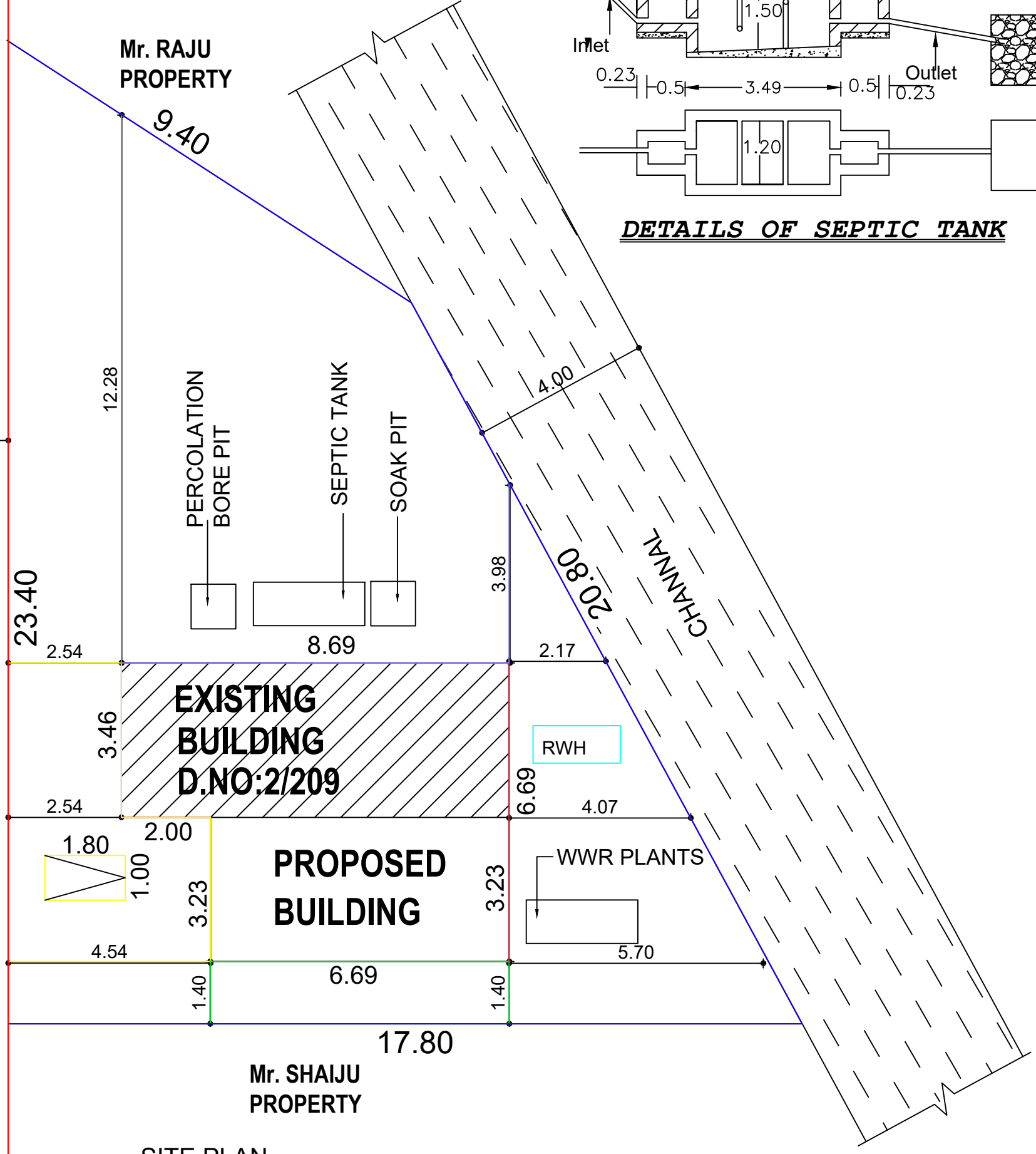
SITE PLAN SCALE 1:100 ALL DIMENSIONS ARE IN METRE
