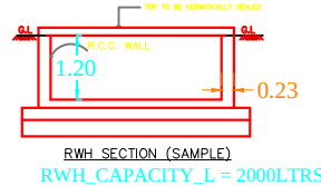
RWHS_SECTION (SAMPLE) RWHS_CAPACITY_L = 2000LTRS
