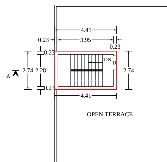
PLAN OF HEAD ROOM FLOOR
