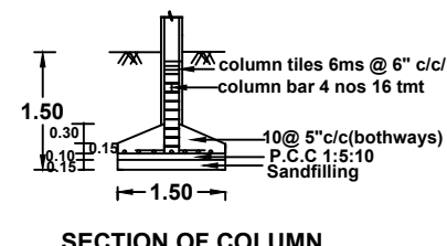
SECTION OF COLUMN
