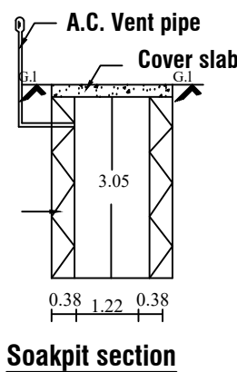
Soakpit section
