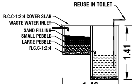
RECYCLING OF WASTE WATER
