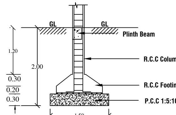
SECTION OF COLUMN
