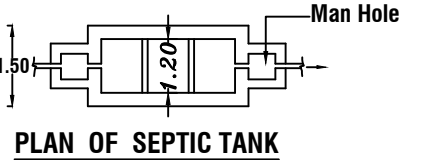
PLAN OF SEPTIC TANK
