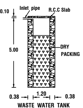
WASTE WATER TANK
