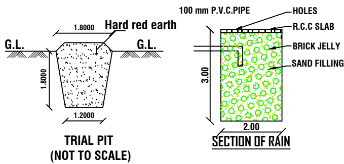
TRIAL PIT (NOT TO SCALE)
