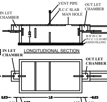
PLAN : SEPTIC TANK NOT TO SCALE
