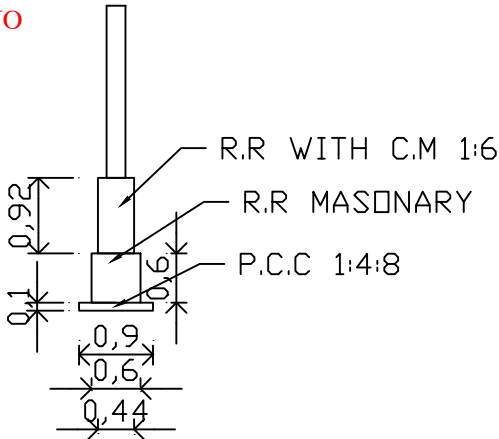
FOUNDATION
