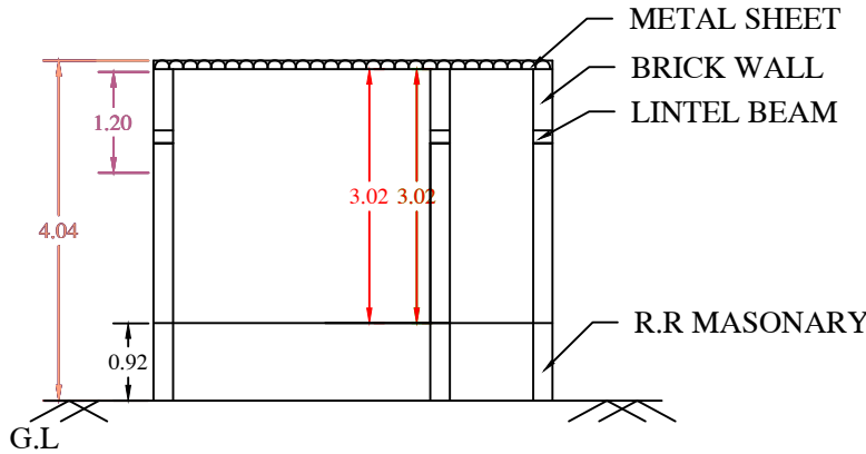
SECTION AT X-X'
