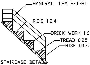
STAIRCASE DETAIL
