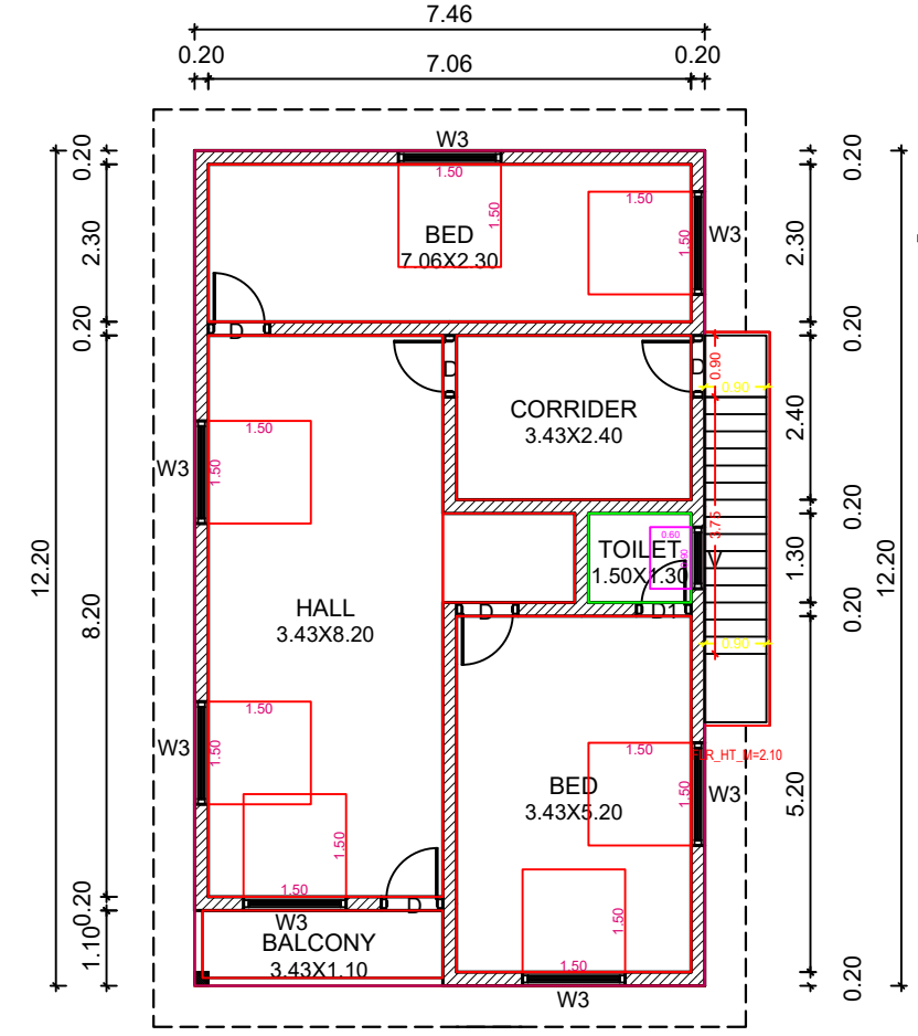
FIRST FLOOR PLAN PROPOSED FLOOR
