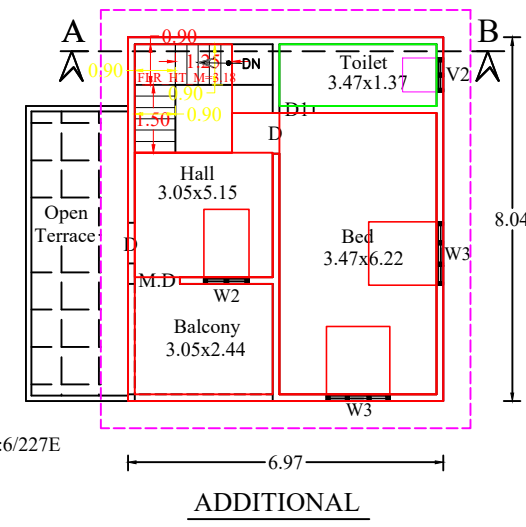
ADDITIONAL FIRST FLOOR PLAN
