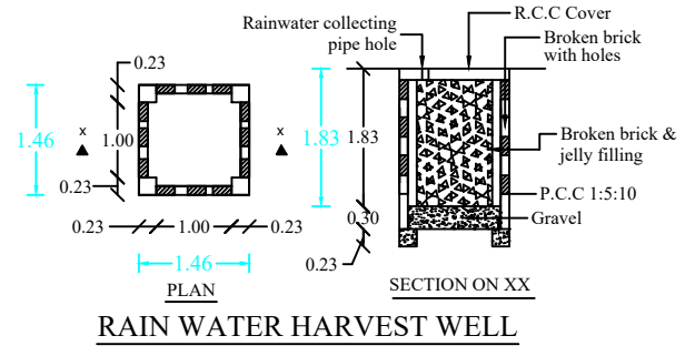
RAIN WATER HARVEST WELL
