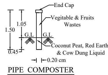
PIPE COMPOSTER
