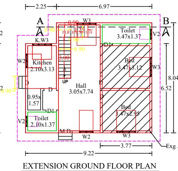
EXTENSION GROUND FLOOR PLAN
