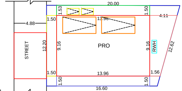
SITE PLAN
