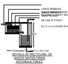
DETAILS OF RECYCLING OF WASTE WATER FROM KITCHEN & TOILET
