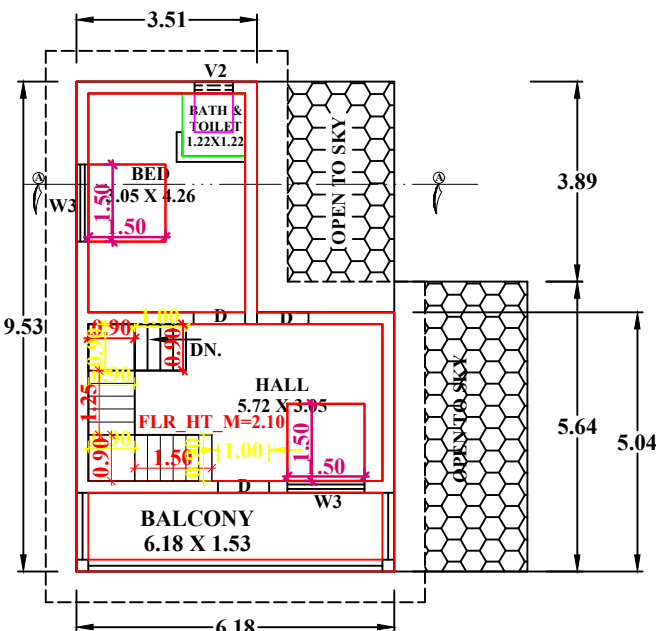
PLAN (FIRST FLOOR)
