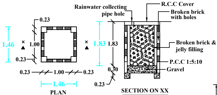
RAIN WATER HARVEST WELL
