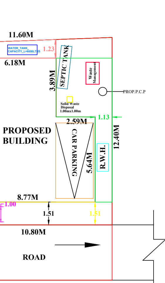
SITE PLAN
