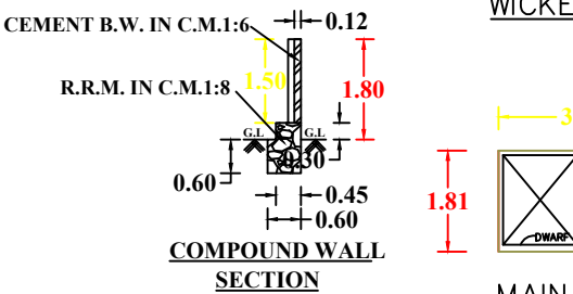
COMPOUND WALL SECTION
