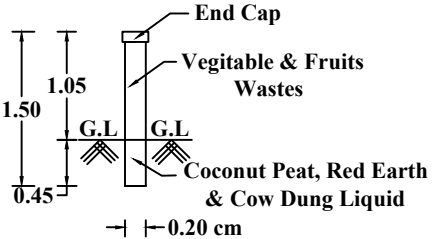
PIPE COMPOSTER
