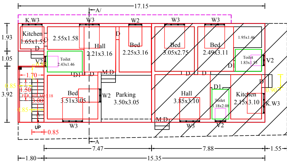
EXISTING & EXTENSION GROUND FLOOR PLAN DOOR NO :- 13-75/2
