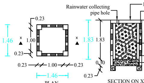
RAIN WATER HARVEST WELL RWH CAPACITY 1=6642LTRS
