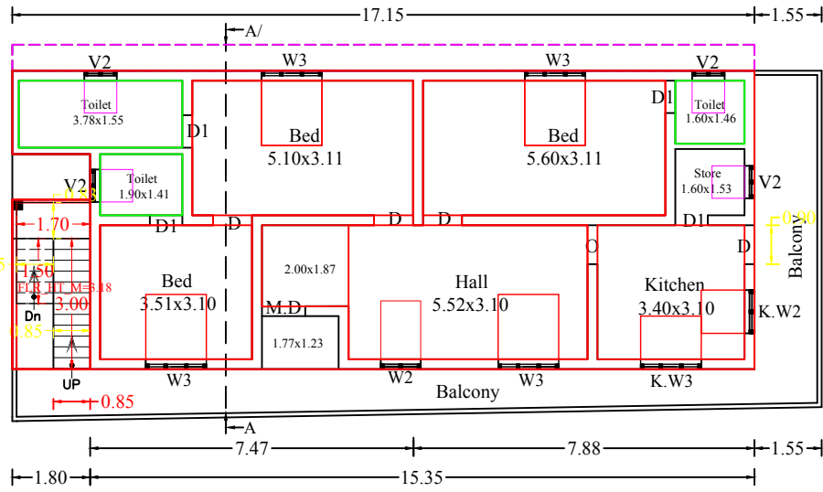
EXTENSION FIRST FLOOR PLAN
