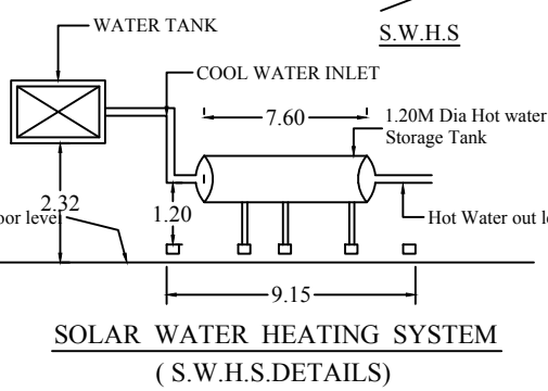
SOLAR WATER HEATING SYSTEM (S.W.H.S.DETAILS)
