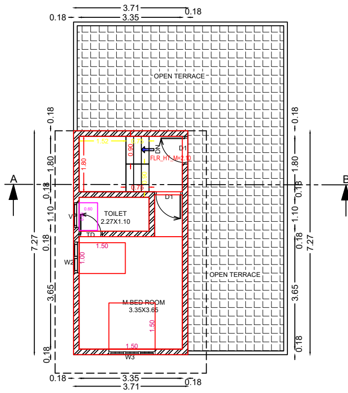
FIRST FLOOR PLAN BUILT UP AREA 27.0 Sq.m (290.52 sq.ft)
