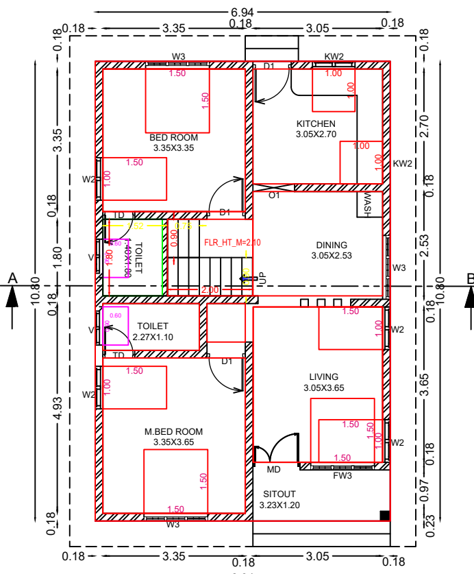
GROUND FLOOR PLAN BUILT UP AREA 75.0 Sq.m (807sq.ft)
