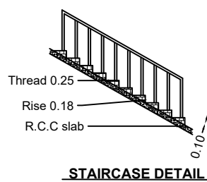
STAIRCASE DETAIL
