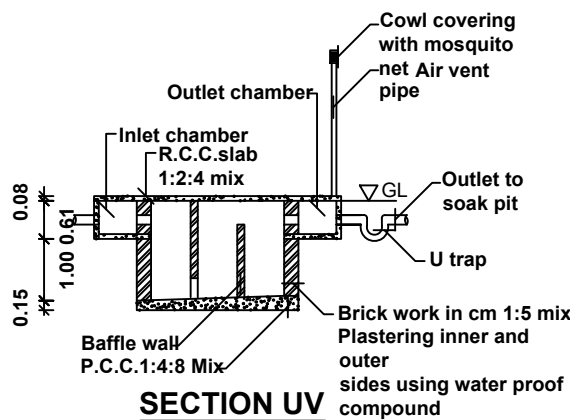
SECTION UV
