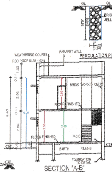
SECTION "A-B"
