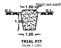
TRIAL PIT (Scale 1:100)
