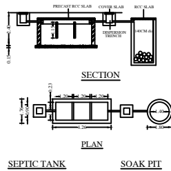
SEPTIC TANK
