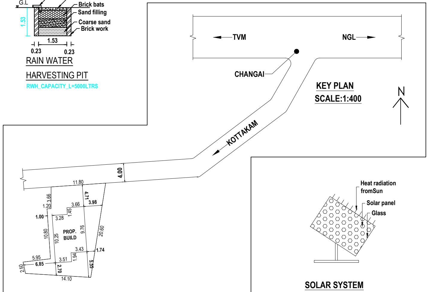
SOLAR SYSTEM
