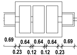
SEPTIC TANK PLAN
