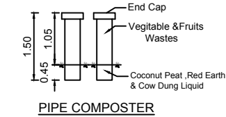
PIPE COMPOSTER
