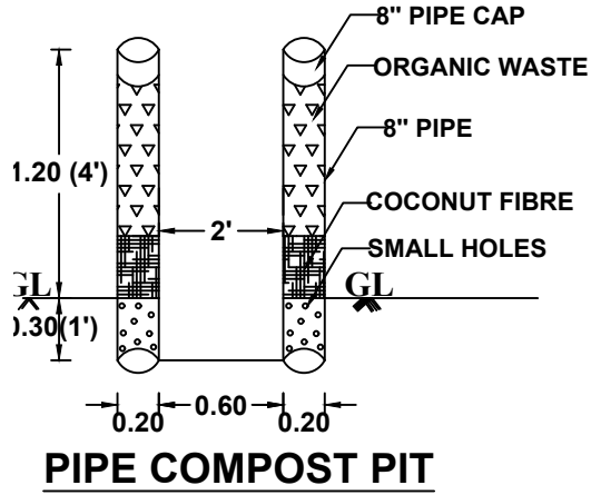
PIPE COMPOST PIT
