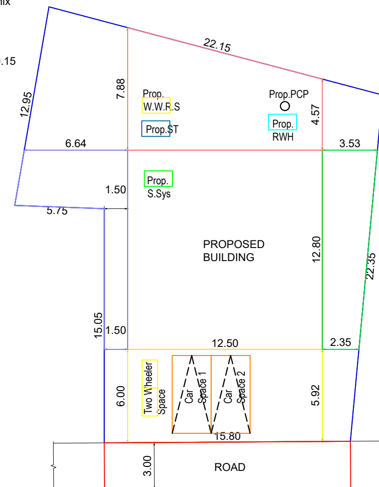
SITE PLAN
