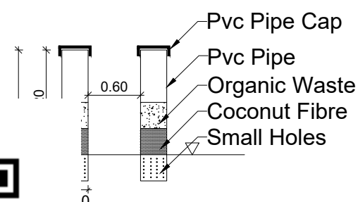
COMPOST PIT
