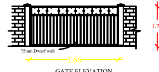
GATE ELEVATION
