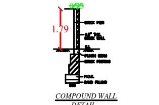
COMPOUND WALL DETAIL
