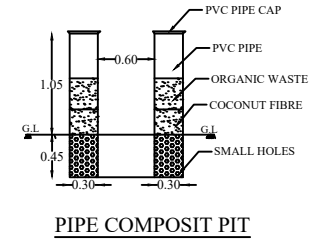
PIPE COMPOSIT PIT
