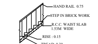
STAIR CASE SECTION
